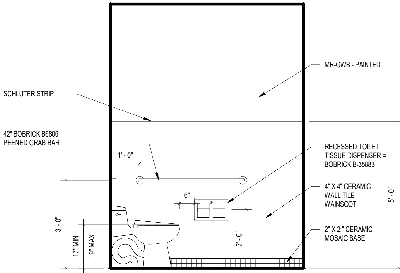
① TOILET - WEST - AMENDED PERMIT 1/2" = 1'-0"
